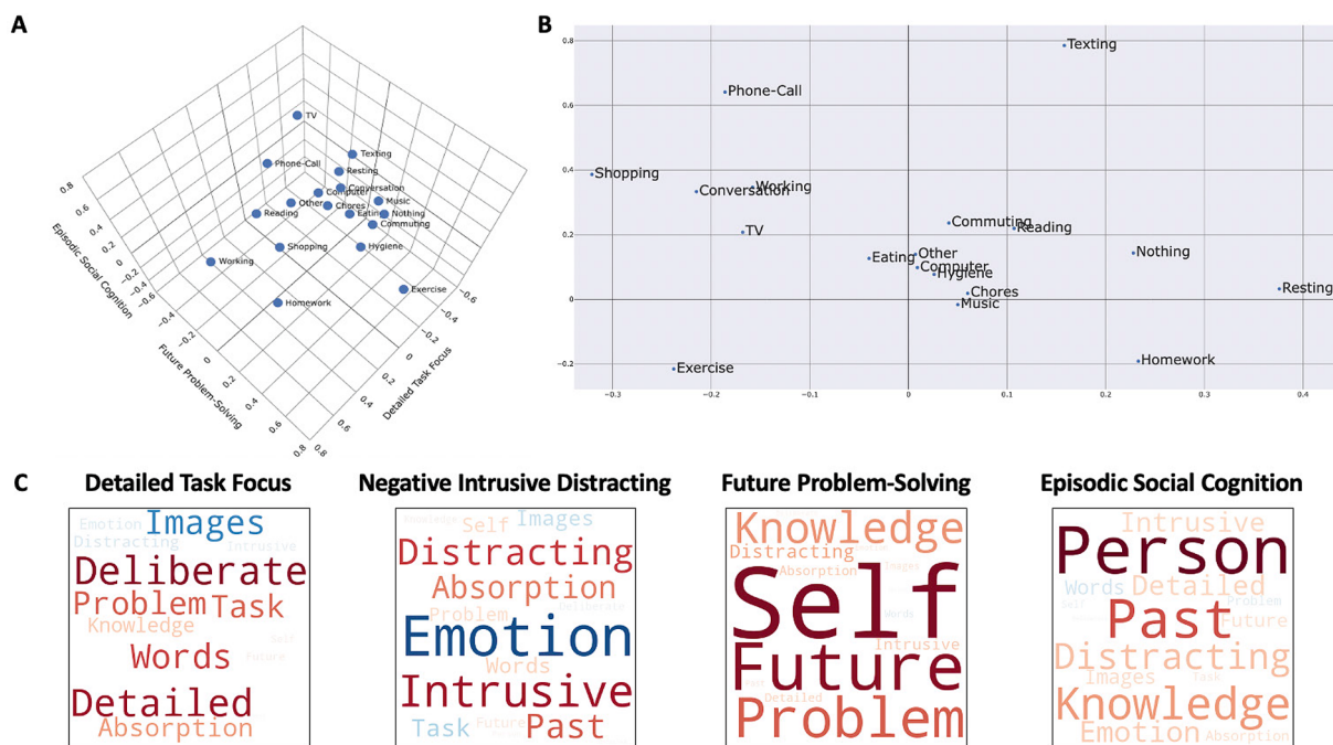
Fig. 5. Mappings between thought patterns and activities in daily life. These data are presented in (A) three- and (B) two-dimensional spaces to provide the opportunity to visualize the relationships between activities and multiple dimensions identified in our study in a convenient way. (B) “Episodic social cognition” component loadings can be found on the y-axis, and “negative intrusive distracting” component loadings can be found on the x-axis. (C) Thought word clouds. Words represent PCA (varimax) scores for MDES dimensions. Larger fonts are items with more importance (i.e., higher loadings) and colour denotes direction (i.e., warm colours relate to positive loadings).
