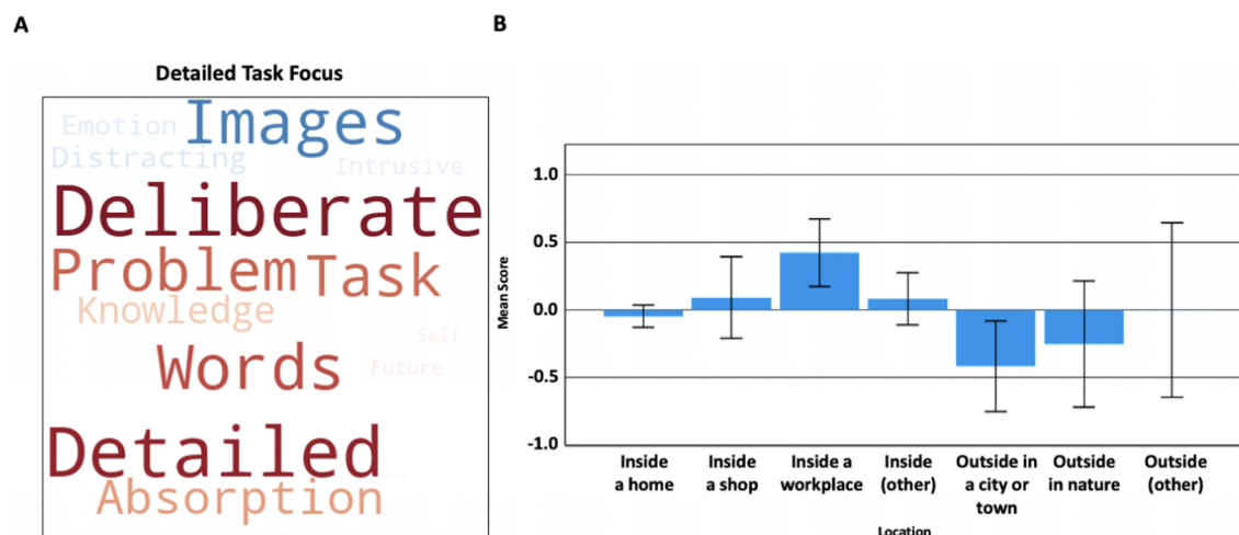
Fig. 6. The influence of location on ongoing thought patterns. (A) “Detailed task focus” word cloud. Words represent PCA (varimax) scores for MDES dimensions. Larger fonts are items with more importance (i.e., higher loadings) and colour denotes direction (i.e., warm colours relate to positive loadings). (B) Bar chart comparing mean MDES scores when participants reported they were 1) inside a home, 2) inside a shop, 3) inside a workplace, 4) inside (other), 5) outside in a city or town, 6) outside in nature, and 7) outside (other). Error bars represent 99 % CIs.
