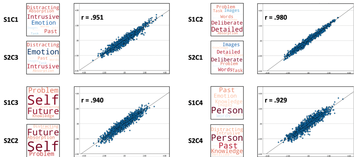
Fig. 2. 4-component solution reliability analysis. Scatter plot of average homologue similarity. “S” indicates subset, and “C” indicates component. Component scores for subset 1 are found on the y-axes and component scores for subset 2 are found on the x-axes.
