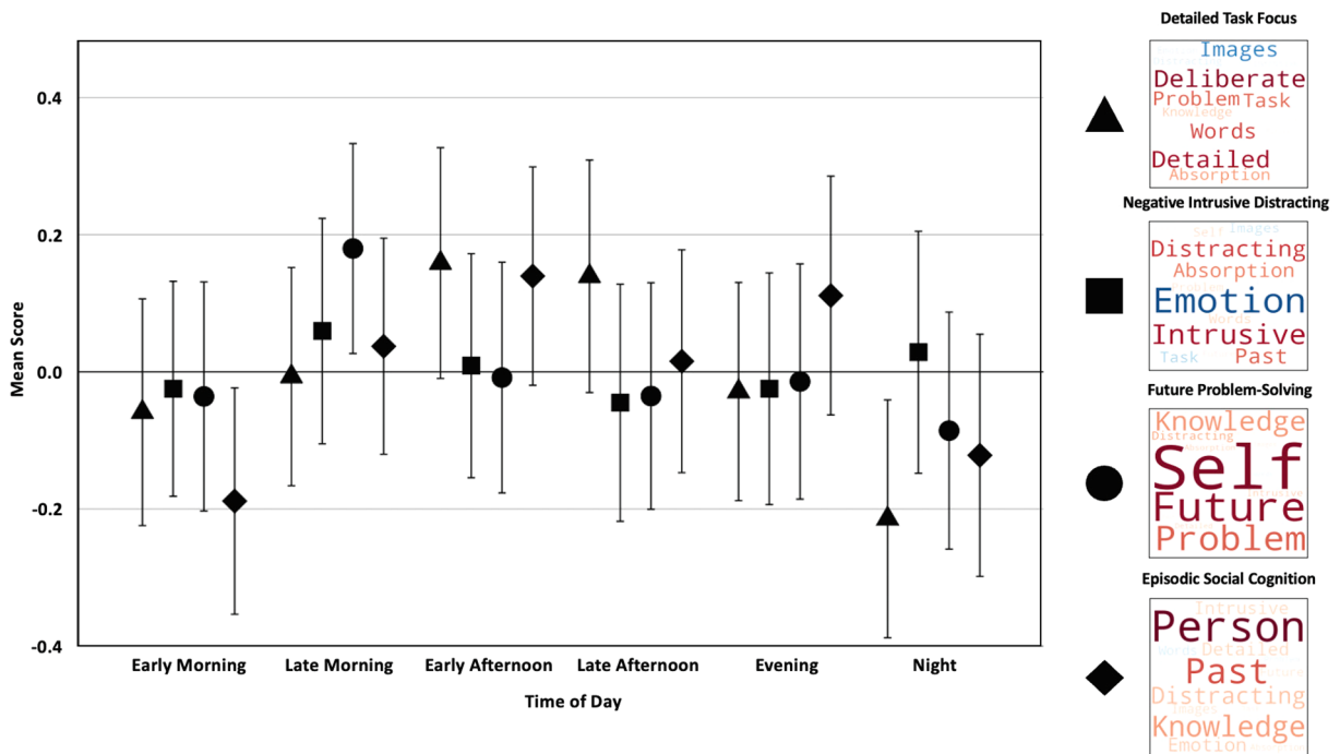
Fig. 7. The influence of time of day on ongoing thought patterns. The graph compares mean MDES scores across different time intervals. “Early morning” = 00:00–10:26:40, “late morning” = 10:33:20–12:26:40, “early afternoon” = 12:33:20–15:06:40, “late afternoon” = 15:13:20–17:40:00, “evening” = 17:46:40–20:26:40, and “night” = 20:33:20–23:53:20. Error bars represent 99 % CIs.
