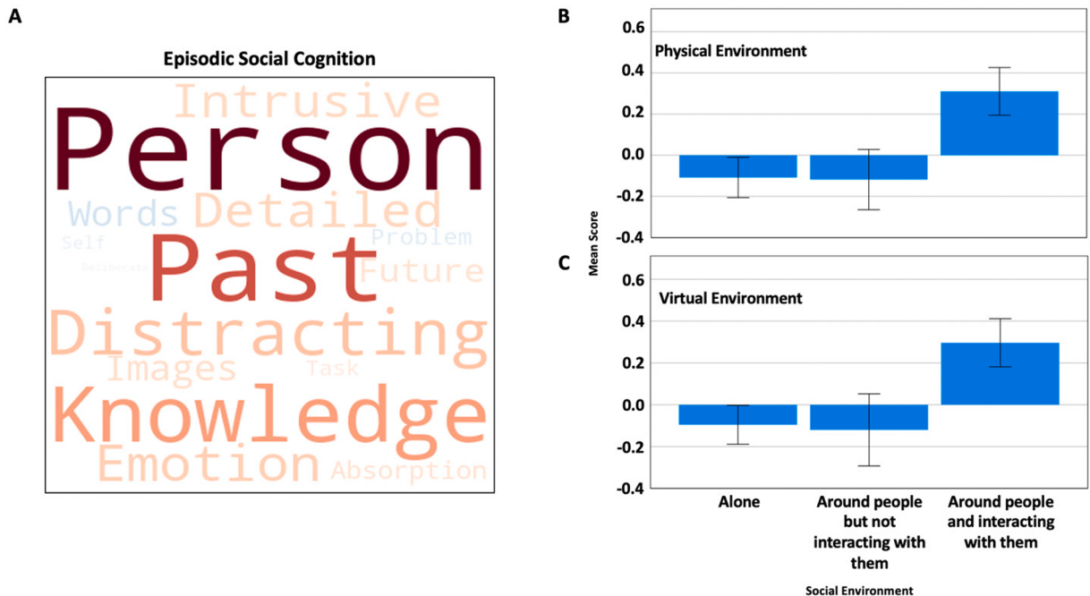
Fig. 3. The influence of socializing on ongoing thought. (A) “Episodic social cognition” word cloud. Words represent PCA (varimax) scores for MDES dimensions. Larger fonts are items with more importance (i.e., higher loadings) and colour denotes direction (i.e., warm colours relate to positive loadings). (B) Bar chart comparing mean MDES scores when participants reported they were 1) alone, 2) physically around people but not interacting with them, and 3) physically around people and interacting with them. Error bars represent 99 % CIs. (C) Bar chart comparing mean MDES scores when participants reported they were 1) alone, 2) virtually around people but not interacting with them, and 3) virtually around people and interacting with them. Error bars represent 99 % CIs.
