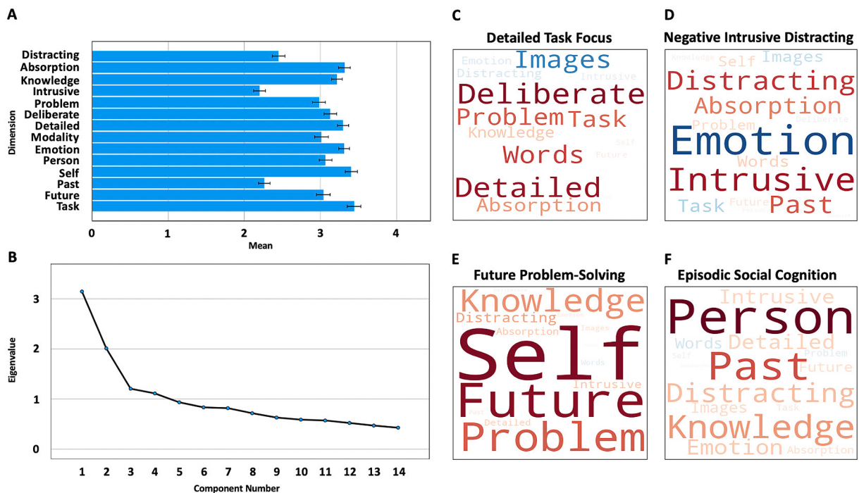
Fig. 1. Patterns of ongoing thought identified through PCA on thought data. (A) Horizontal bar graph of mean dimension scores. Error bars represent 99 % confidence intervals (CIs). (B) Scree plot generated from PCA of MDES data. (C-F) Thought word clouds. Words represent PCA (varimax) scores for MDES dimensions. Larger fonts are items with more importance (i.e., higher loadings) and colour denotes direction (i.e., warm colours relate to positive loadings). (C) “Detailed task focus” word cloud. (D) “Negative intrusive distracting” word cloud. (E) “Future problem-solving” word cloud. (F) “Episodic social cognition” word cloud.
