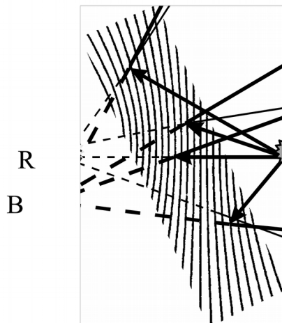
Figure 1.13: Dispersion in an off-axis reflection hologram: The broad band illumination source point to the right results in Red and Blue image points to the left.
