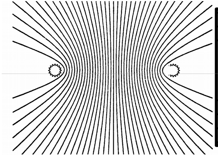
Figure 1.5: Interference pattern forming a Gabor zone plate
