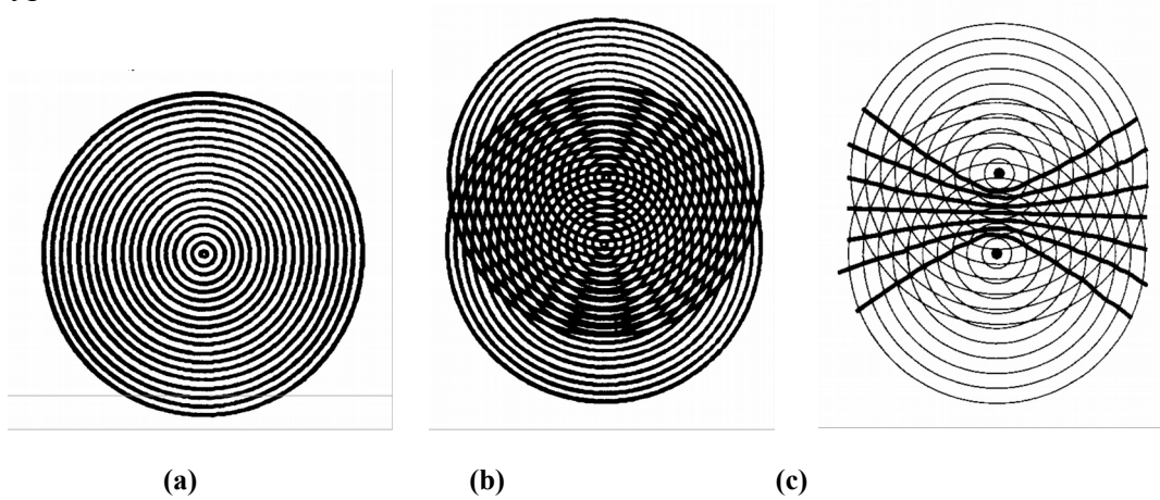
Figure 1.2: The Moire fringe pattern is a helpful visual aid to understanding interference effects 2 . Here we have the oscillating source above in isolation, and interfering with another source.
