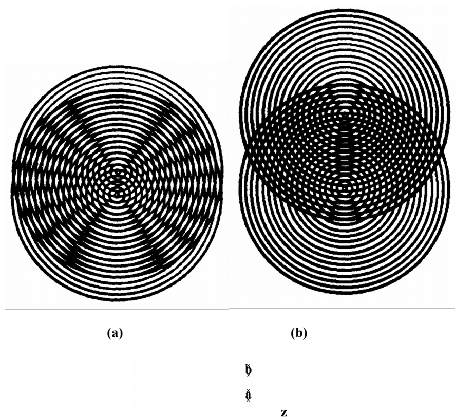
Figure 1.6: As the apparent distance between source points increases, so too does the spatial frequency of the fringes. In this figure, we are looking at the two sources from two different points on the recording material, one point close to the optical ( z -) axis (a), another farther off-axis (b).
