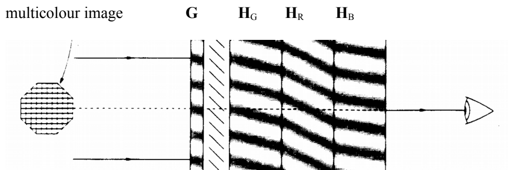
Figure 3.13: Bazargan's suggested approach for making a full-color, dispersion-compensated display
