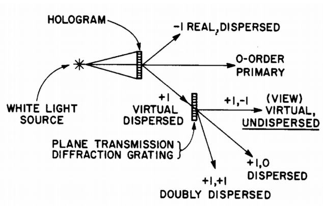
Figure 3.1: DeBitetto's original diagram discriminating the effects of diffraction orders on relative dispersion
