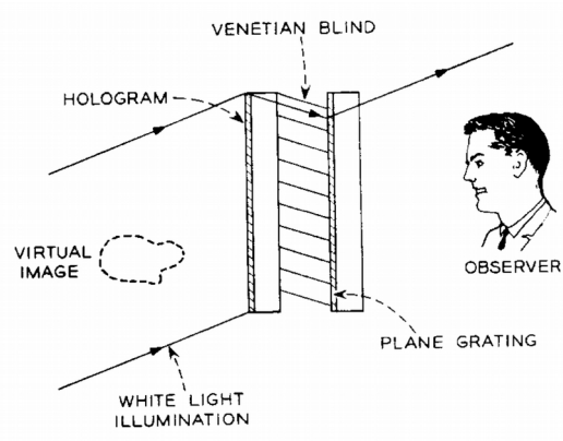
Figure 3.6: Burckhardt's (1966) use of a louver film to block the zero order of the hologram in a single view angle dispersion-compensation display
