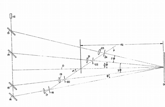
Figure 3.11: Benton's patent drawing of the special achromatizing grating used in an exposure step (1985)
