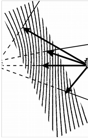
Figure 1.12: Reconstruction of an off-axis reflection hologram, where the twin image is eliminated. The illumination source point is to the right, and the virtual image is to the left.
