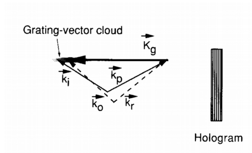
Figure A1.1: Grating vector cloud (Goodman, 1996)
