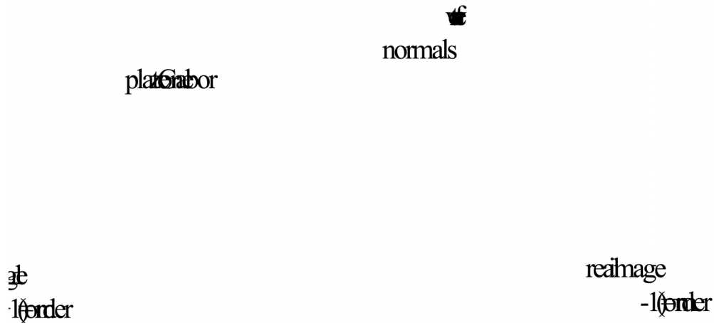
Figure 1.8: Illumination of a Gabor zone plate with a single wavelength, with resulting virtual and real image points
