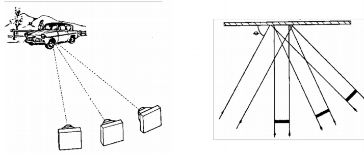
Figure 4.1: Sequential images are taken, and later projected to expose a hologram with an appropriately scaled geometry (Redman 1968).
