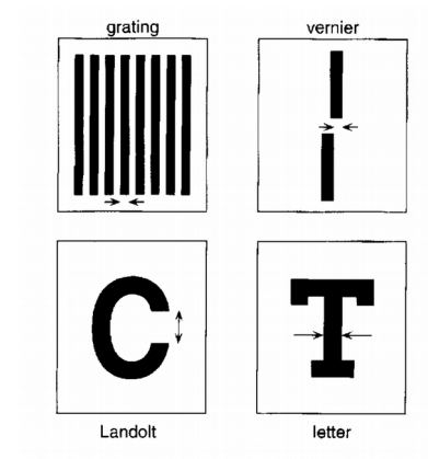
Figure 1.15: Different acuity tests (Geisler and Banks, fig. 7.25.36-19)
