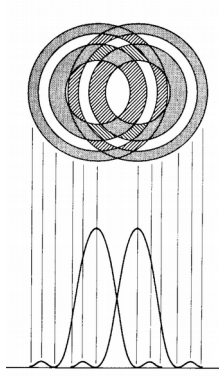
Figure 1.18: Rayleigh’s criterion for just resolvable points. Here are two overlapping Airy disk patterns, the images of two closely spaced points. As in Figure 1.17, the lines merely ascribe areas of the diffracted pattern to points on corresponding intensity curves (Riggs 1965, fig. 11.11).
