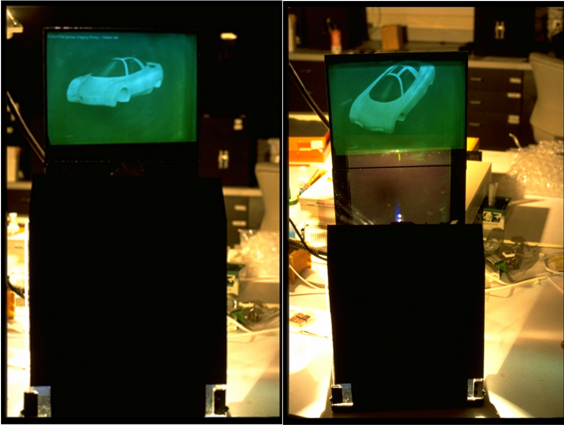
Figure 5.10: Plane-wave grating dispersion-compensation display (photos care of Michael Klug)
