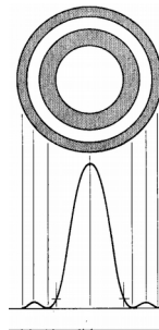
Figure 1.17: Airy disk diffraction pattern. The lines merely ascribe areas of the diffracted pattern to points on the corresponding intensity curve (Riggs 1965, fig. 11.10).
