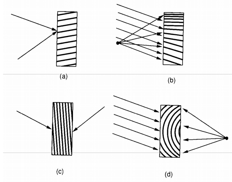
Figure 1.14: Examples of different fringe patterns (Goodman 1996):
