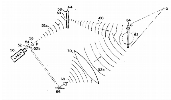
Figure 3.10: Benton's patent drawing of the white-light transmission hologram transfer step (1972)
