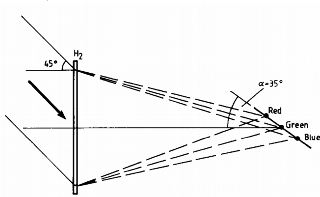
Figure 2.6: Wavelength-dependent focusing power of a hologram, and the achromatic angle (Saxby 1992)
