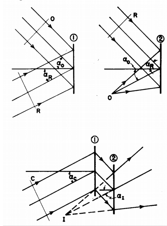
Figure 3.4: A schematic representing the original geometry of the three researchers in reverse (Latta 1972) (1) is an off-axis plane-wave grating, and (2) is a hologram to be illuminated at the output angle of (1).
