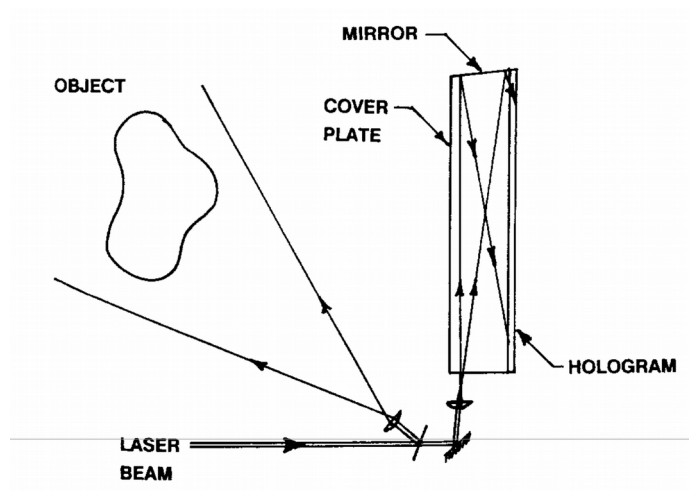
Figure 6.2: Exposure of an edgelit hologram illuminated with the same source distance and folded beam path (Upatnieks 1992)
