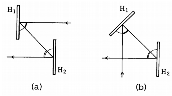
Figure 3.14: Kubota's reflection /reflection dispersion-compensated display
