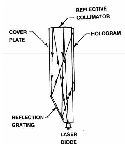
Figure 6.4: Upatnieks' achromatic edgelit hologram (1992)
